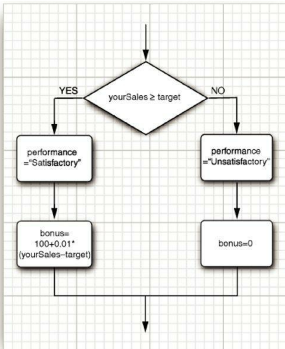
Figure 3.8. Flowchart for the if/else statement
