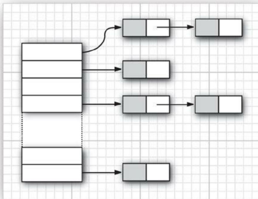
Figure 13.8. A hash table
