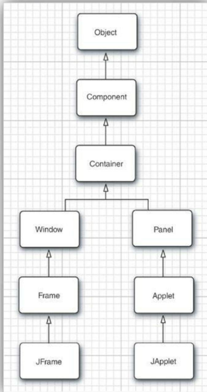
Figure 10.11. Applet inheritance diagram
