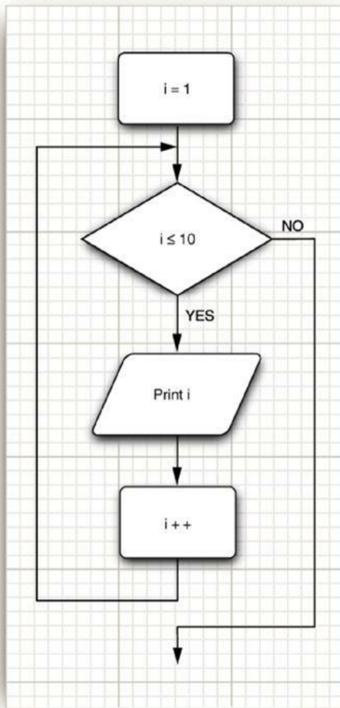
Figure 3.12. Flowchart for the for statement
