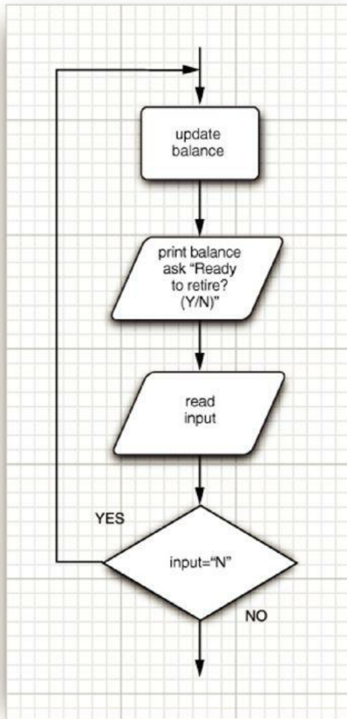
Figure 3.11. Flowchart for the do/while statement
