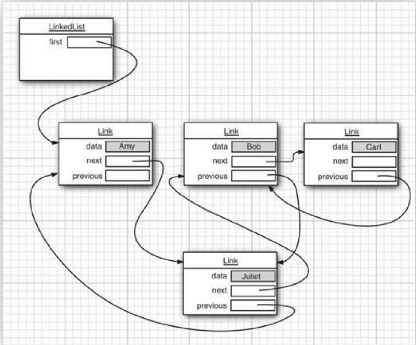
Figure 13.7. Adding an element to a linked list
