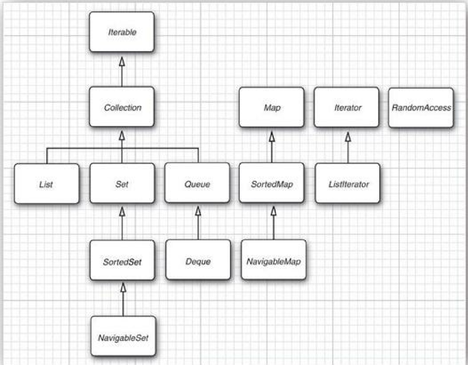
Figure 13.10. The interfaces of the collections framework
