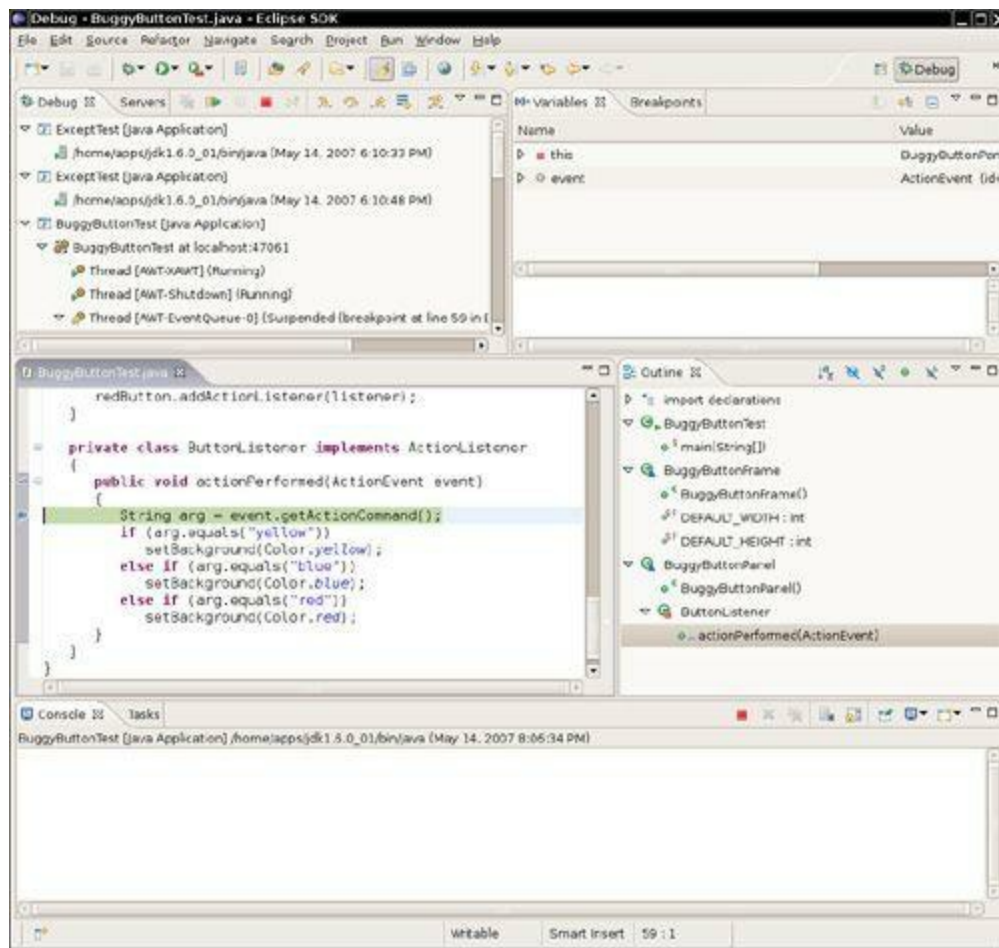
Figure 11.6. Stopping at a breakpoint
