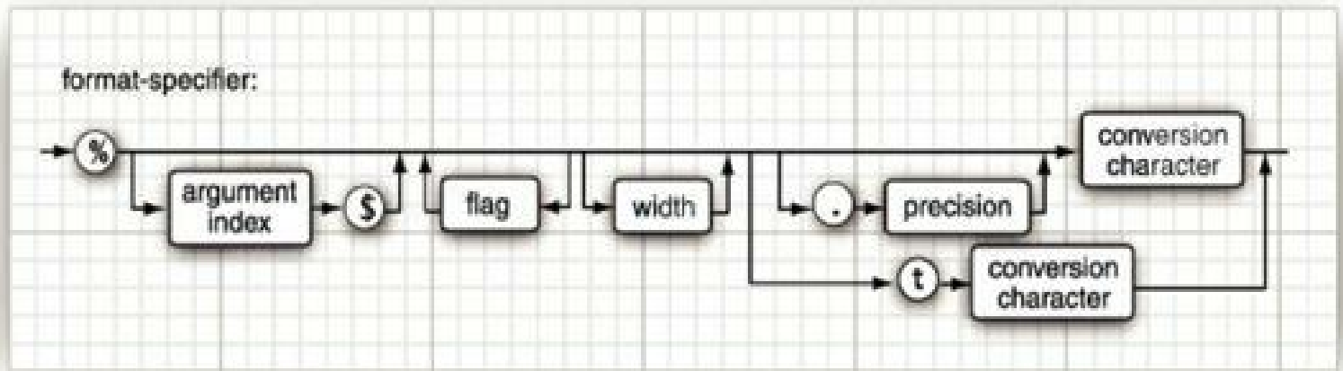
Figure 3.6. Format specifier syntax
