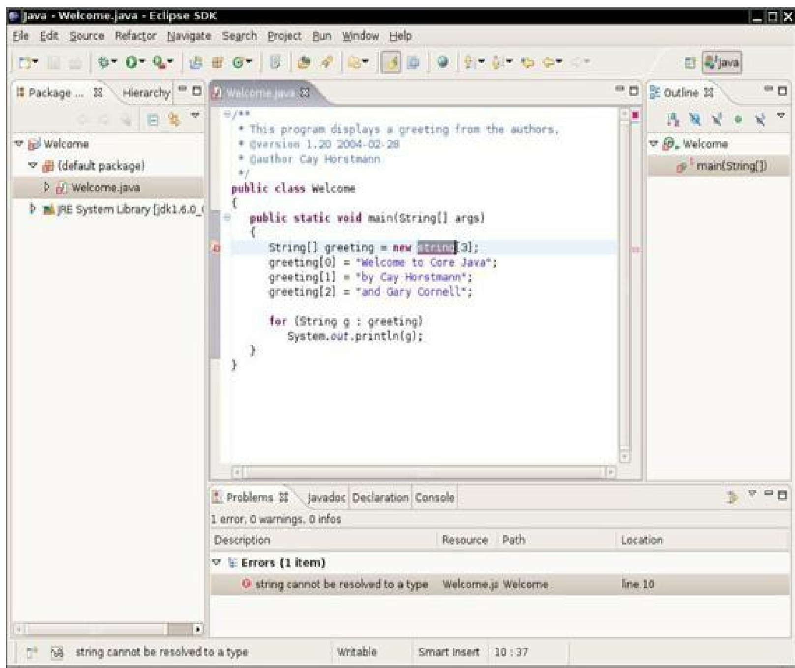
Figure 2.9. Error messages in Eclipse
