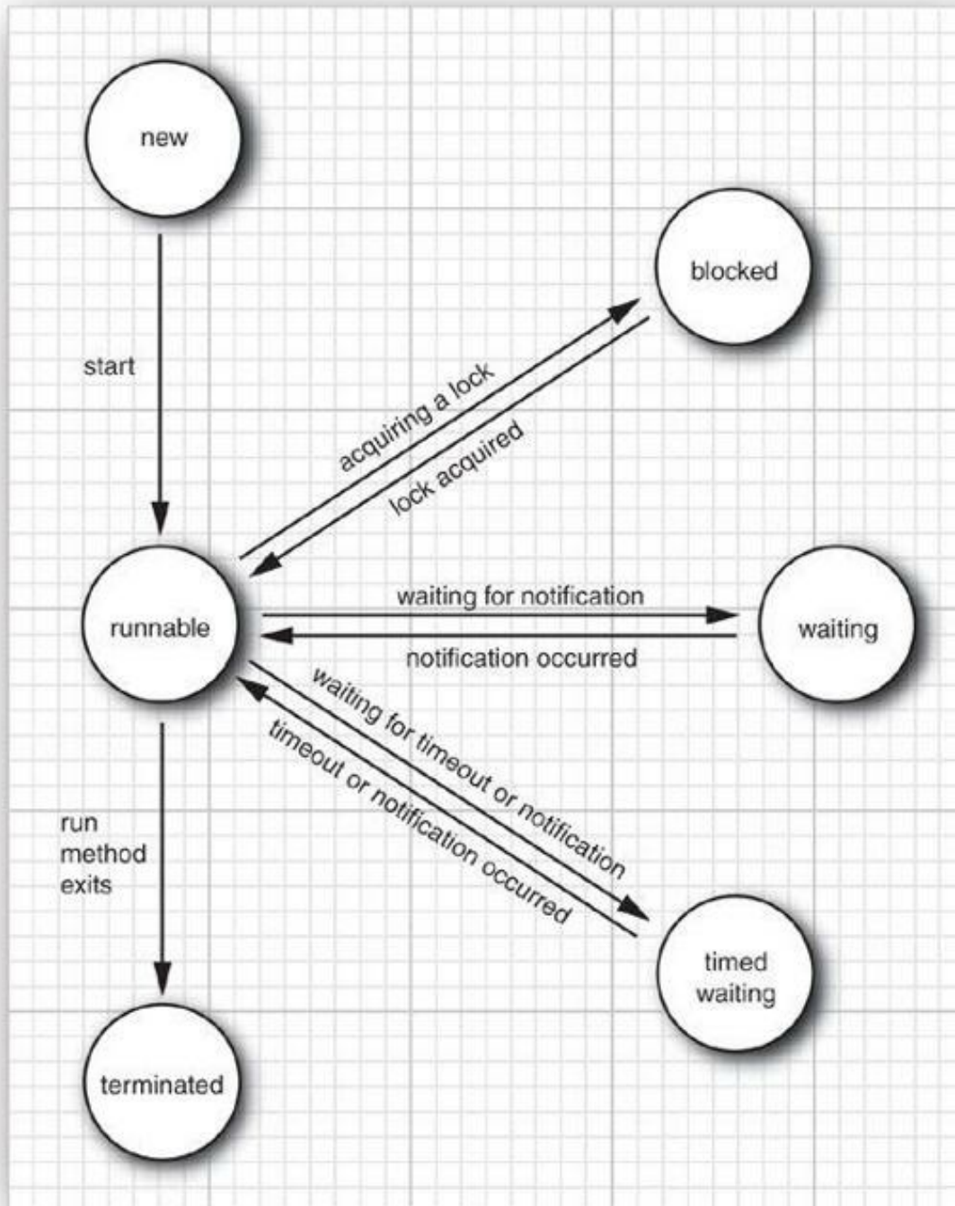
Figure 14.3. Thread states
