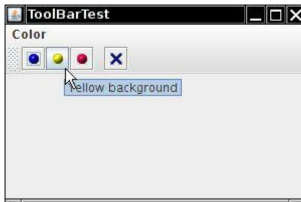
Figure 9.28. A tooltip
