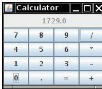
Figure 9.12. A calculator
