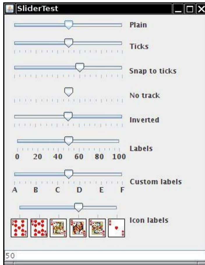
Figure 9.18. Sliders
