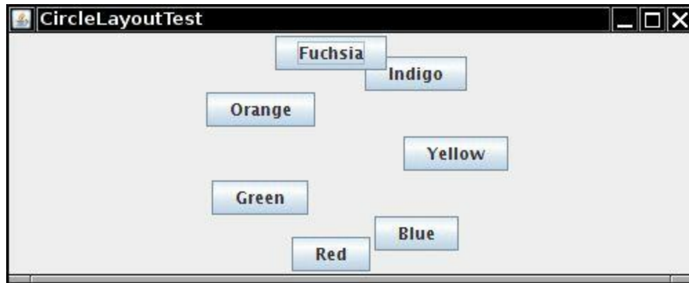
Figure 9.34. Circle layout
