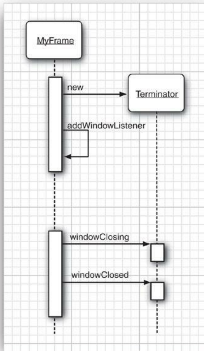
Figure 8.5. A window listener
