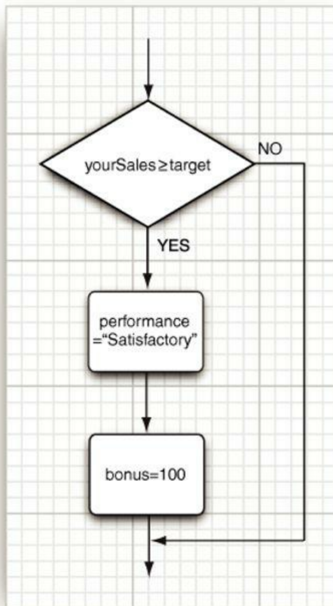
Figure 3.7. Flowchart for the if statement
