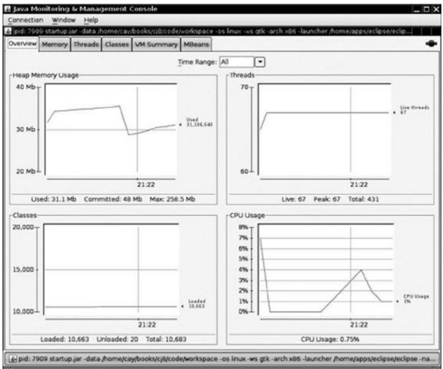
Figure 11.3. The jconsole program
