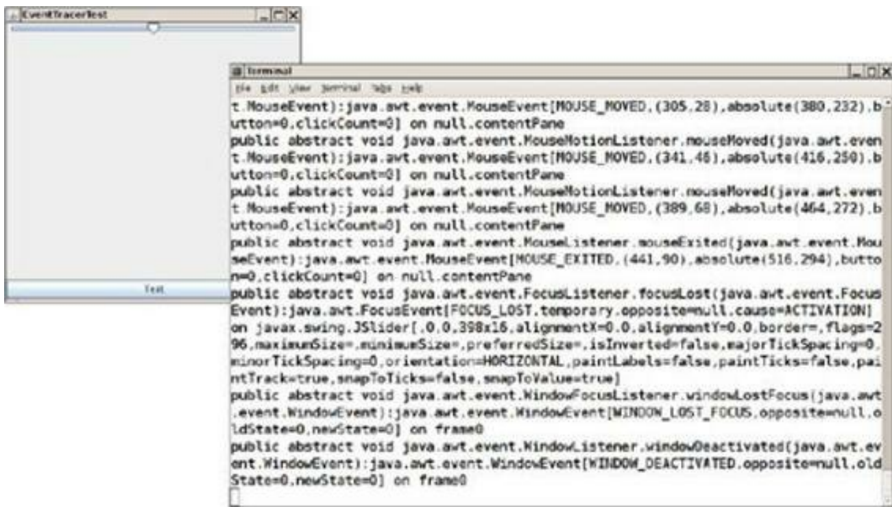
Figure 11.4. The EventTracer class at work
