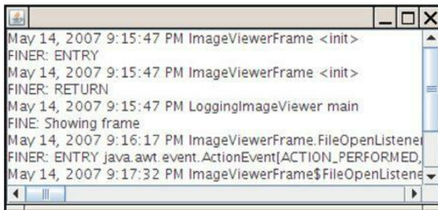
Figure 11.2. A log handler that displays records in a window
