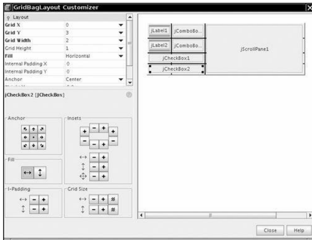
Figure 9.31. Specifying grid bag constraints in NetBeans
