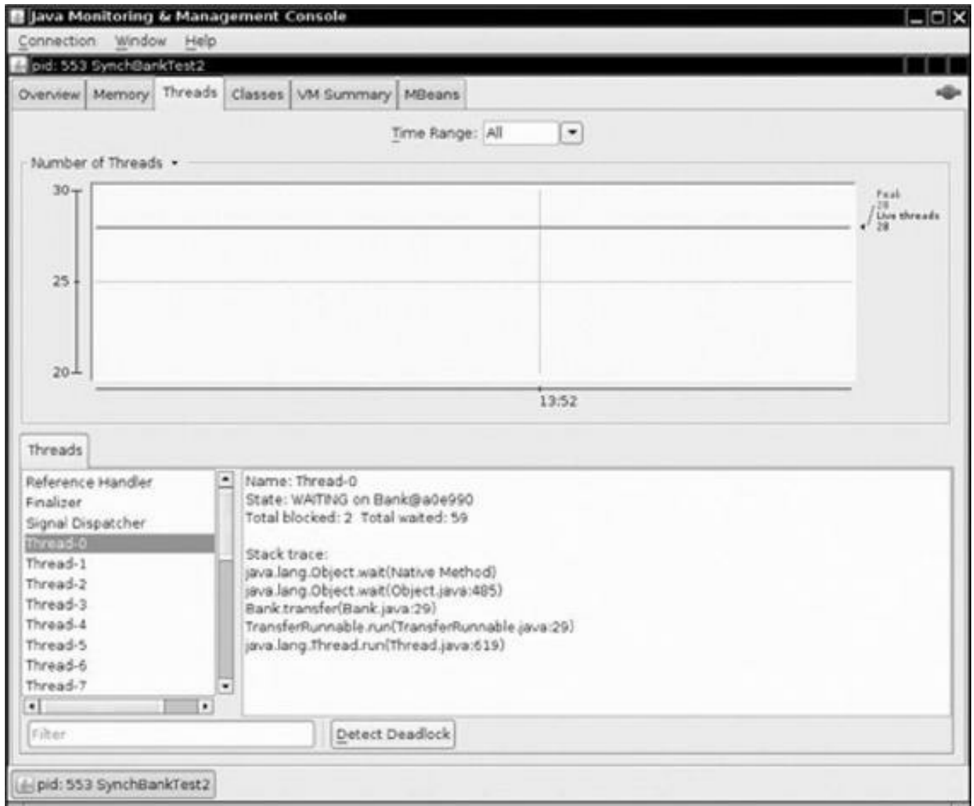
Figure 14.7. The Threads panel in jconsole
