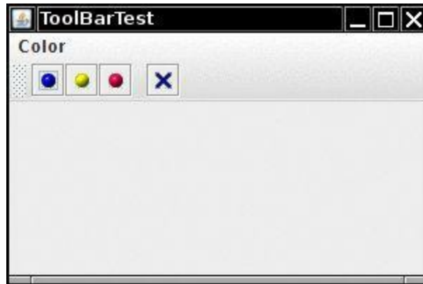
Figure 9.24. A toolbar
